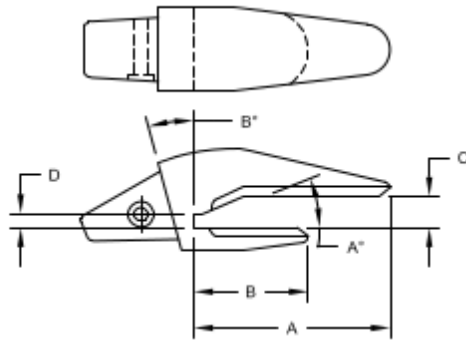
CENTER W/O LOADER ADAPTER
