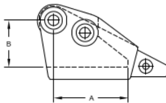
BOLT ON CORNER ADAPTER (2 Bolts)
