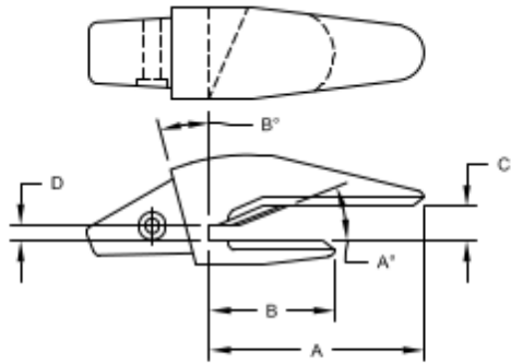
RH W/O LOADER ADAPTER
