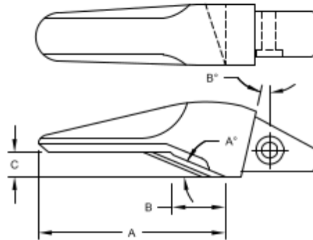
LH-SPADE W/O ADAPTER
